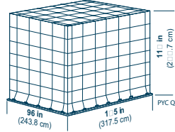
IATA ULD code: PYB Q7 Universal general-purpose flat pallet for lower holds and main decks.
