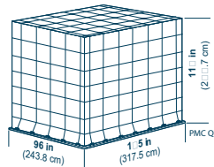
IATA ULD code: PMC Q7 Universal general-purpose flat pallet for lower holds and main decks. Tare weight: 120 kg (265 lb) Volume: H 299.7 cm (118 in), 21.2 m 3 (750 ft 3 )
