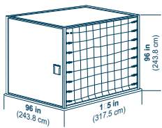
ULD code: AMA rectangular container on P6P base Main-deck container. Door is canvas with built-in net door straps. Maximum gross weight: 6,804 cm (15,000 lb) Tare weight: 350 kg (772 lb),
