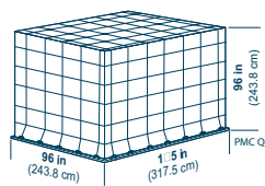
IATA ULD code: PMC Q6 Universal general-purpose flat pallet for lower holds and main decks. Tare weight: 120 kg (265 lb) Volume: H 243.8 cm (96 in), 17.0 m 3 (600 ft 3 )
