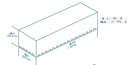
ULD code: AMA rectangular container on P6P base Main-deck container. Door is canvas with built-in net door straps. Maximum gross weight: 6,804 cm (15,000 lb) Tare weight: 350 kg (772 lb),
