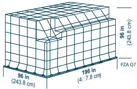
IATA ULD code: PZA Q7 Universal general-purpose flat pallet for lower holds and main decks.
