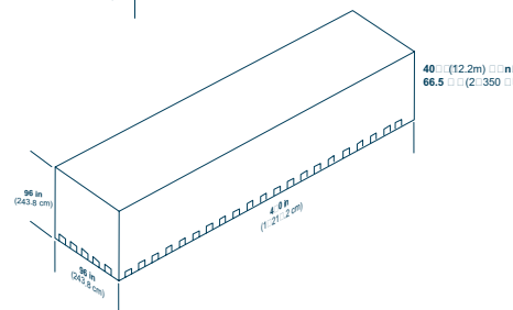
747F nose cargo door only
