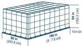
IATA ULD code: PZA Q6 Universal general-purpose flat pallet for lower holds and main decks.
