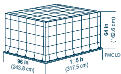
IATA ULD code: PMC LD Universal general-purpose flat pallet for lower holds and main decks. Tare weight: 120 kg (265 lb) Volume: H 162.6 cm (64 in), 11.5 m 3 (407 ft 3 )
