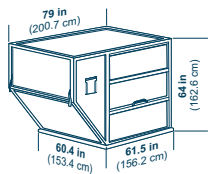
IATA ULD code: AKE contoured container Half-width lower hold container with one angled side. Door is either canvas or solid. Door opening: 58 x 61-in (147 x 155-cm) Maximum gross weight: 1,588 cm (3,500 lb) Tare weight: 82 kg (181 lb) AS1825 volume: 4.5 m 3 (159 ft 3 )
