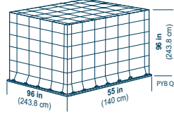
IATA ULD code: PYB Q6 Universal general-purpose flat pallet for lower holds and main decks.
